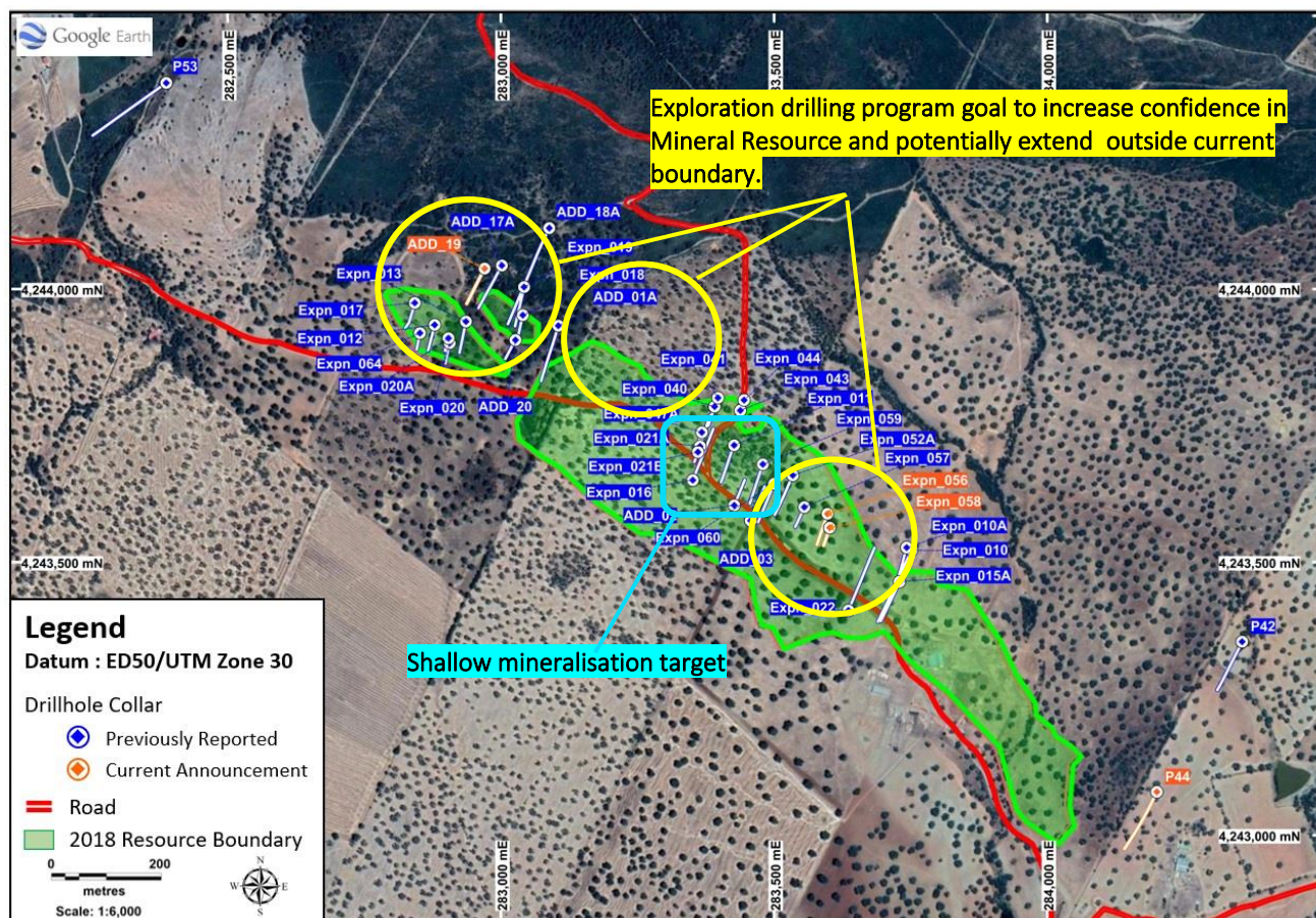
Figure 1. Location of drill holes with reported assay data as at 11th August 2021, from the exploration drilling program at the Oropesa Tin Project, Spain
