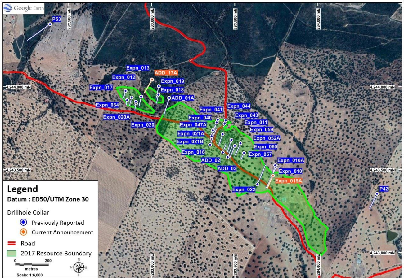
Figure 2. Location of drill holes with assay data as at 16 th June 2021, from the exploration drilling program at the Oropesa Tin Project, Spain
