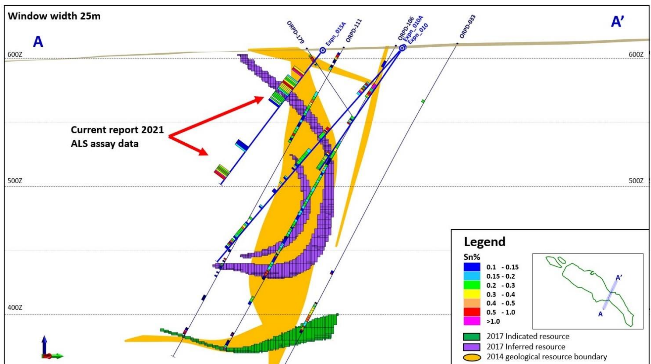
Figure 3. Oropesa 2021 resource infill diamond drilling, Exprn_015A
