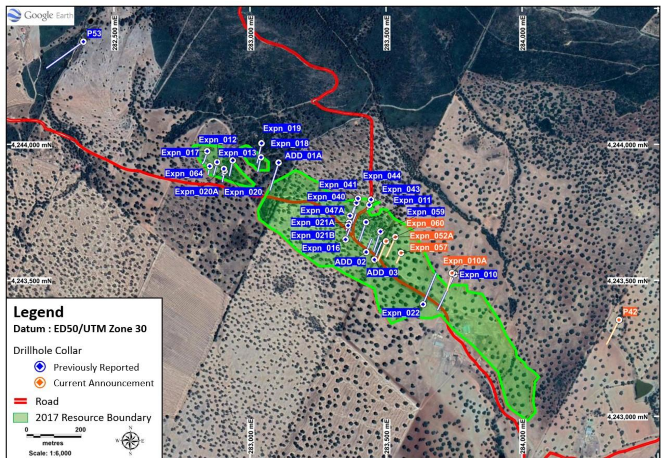
Figure 2. Location of drill holes with assay data as at 2 nd June 2021, from the exploration drilling program at the Oropesa Tin Project, Spain
