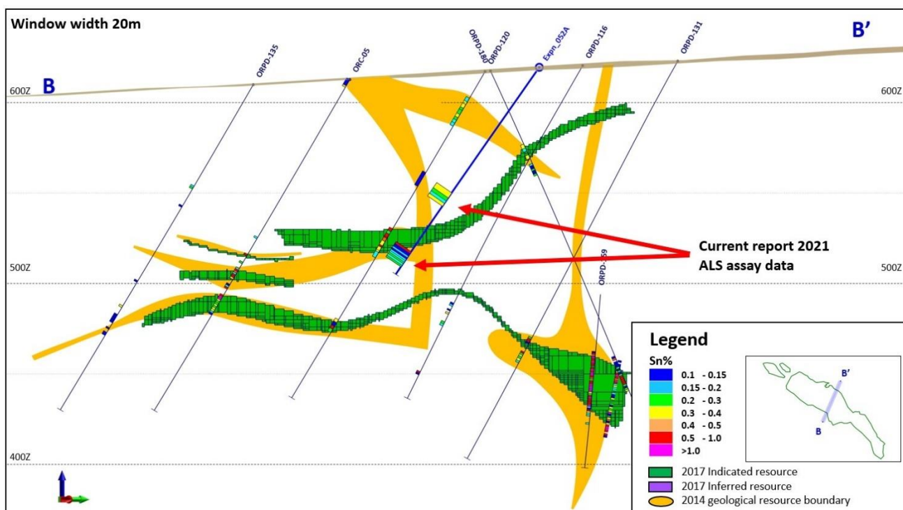
Figure 5. Oropesa 2021 resource infill diamond drilling, Expn_052A
