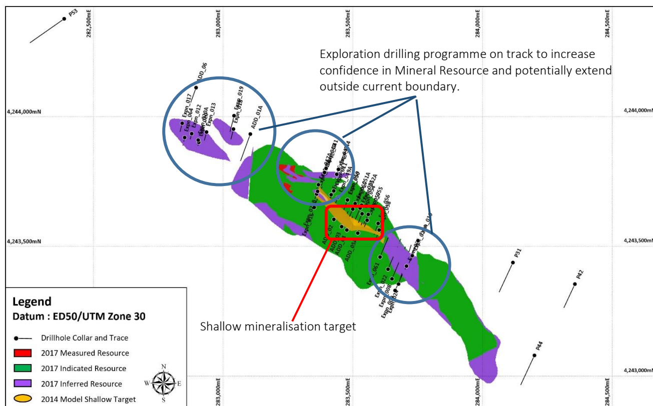
Figure 1. Oropesa geological resource depicting the location of the 2020-21 diamond drilling program.
