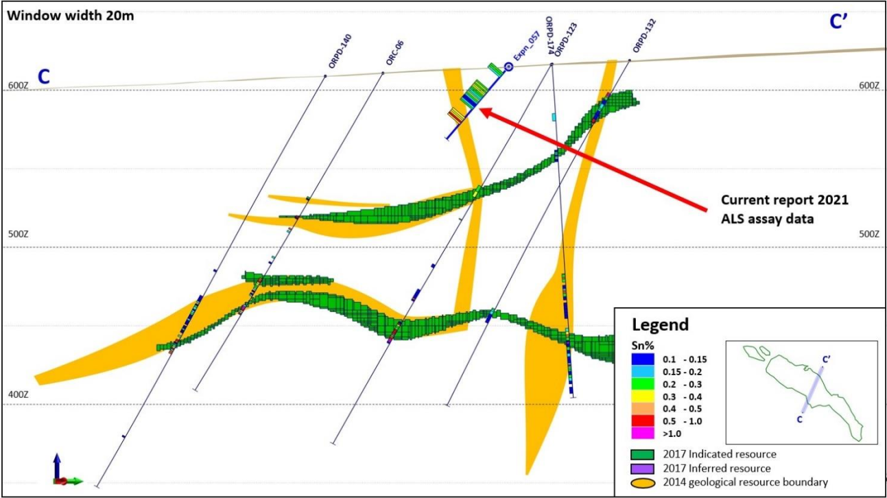
Figure 6. Oropesa 2021 resource infill diamond drilling, Expn_057
