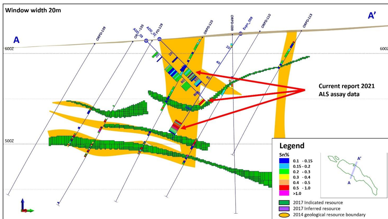
Figure 4. Oropesa 2021 resource infill diamond drilling, ADD-02, ADD_03 & Expn_059
