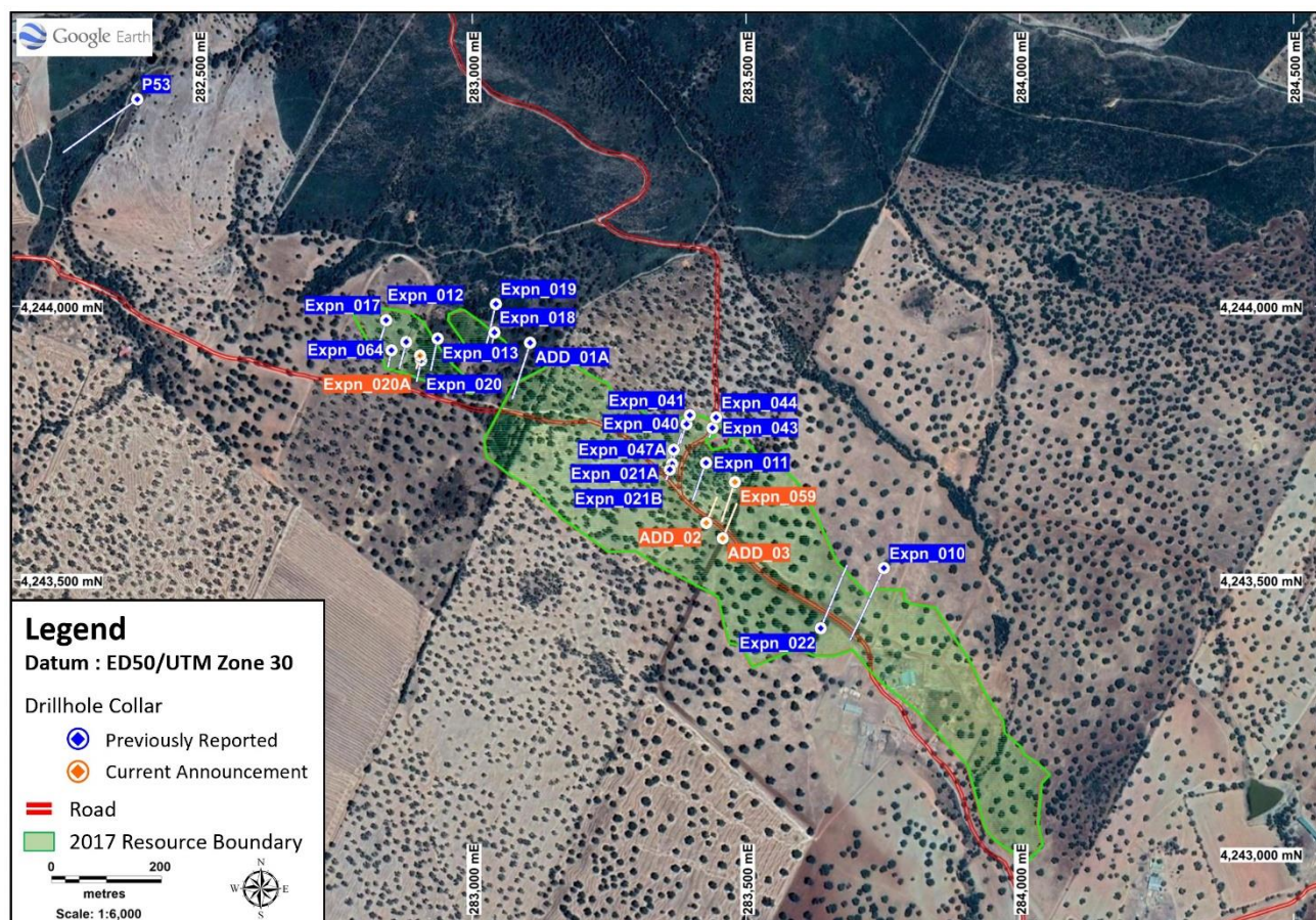
Figure 2. Location of drill holes with assay data as at 29 th April 2021, from the exploration drilling program at the Oropesa Tin Project, Spain
