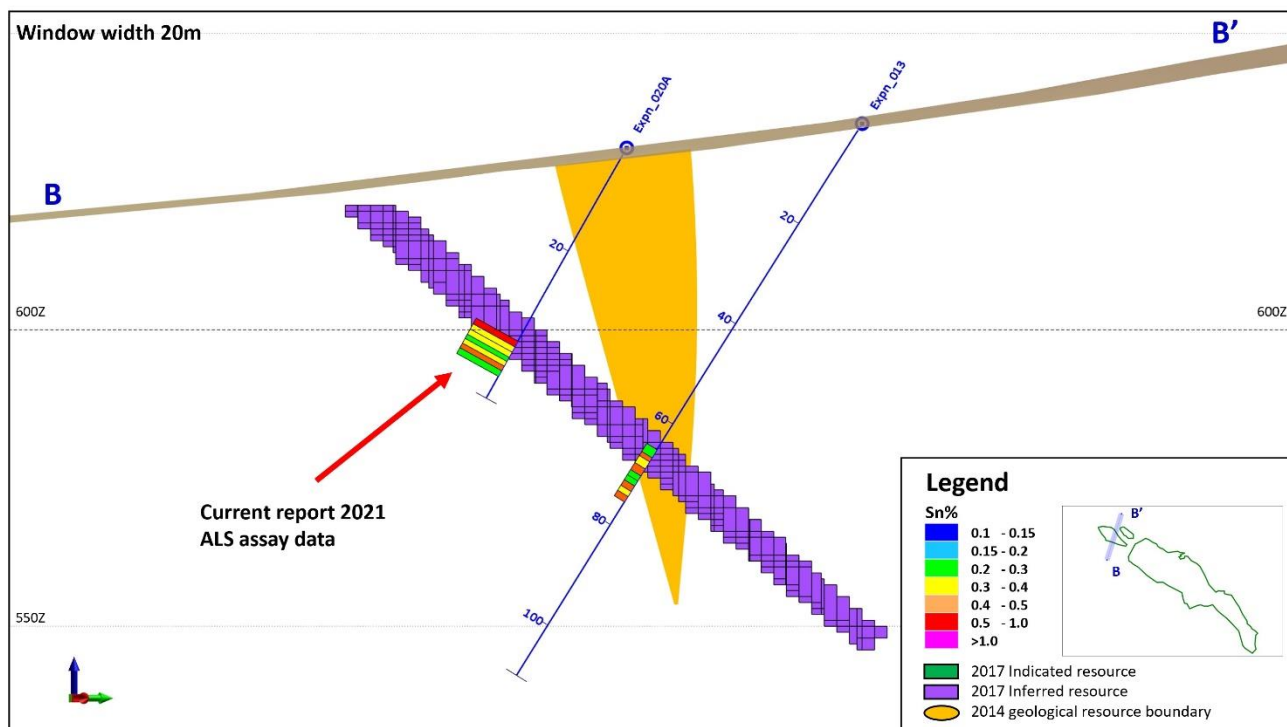
Figure 3. Oropesa 2021 resource infill diamond drilling, Expn_020A.
