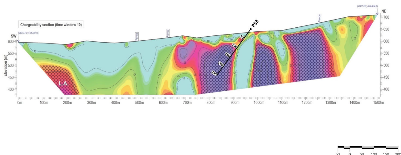
Figure 5. Cross-section of the location of Exploration drill hole P53 overlain on section of chargeability for IP line W4
