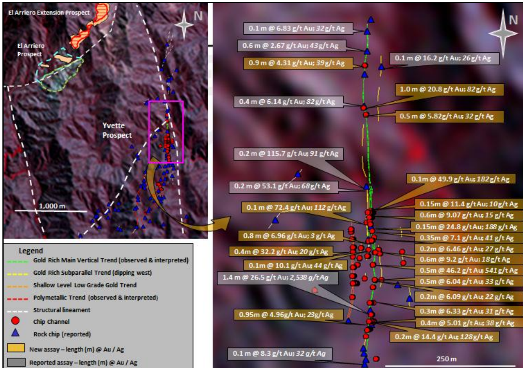
Figure 1: Yvette project. Locations of channel sample intersections with gold and silver grades. Because of talus soil coverage, non-exposed vein segments between channels samples are interpreted.
