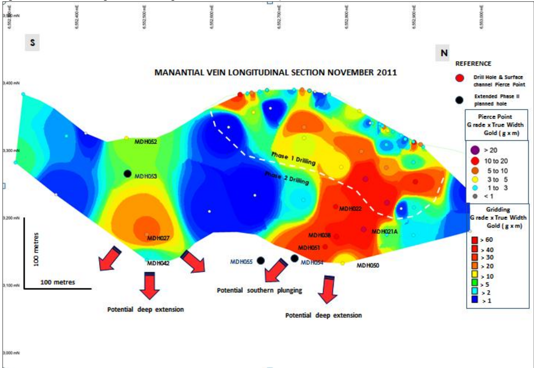
Figure 1: Manantiales long-section showing the location of the three planned drillholes, MDH053, 054 and 055.
